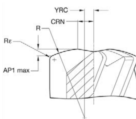
FH200-H schematic diagram of 6 flute endmill shaver blade
